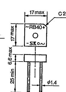
Outline Drawing ㉔
