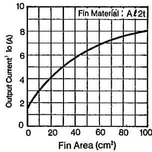
Io - Fin Characteristics
