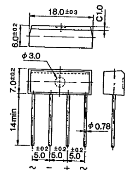
Outline Drawing 22
