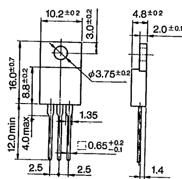
Outline Drawing ⑱
