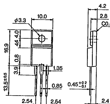
Outline Drawing ⑱
