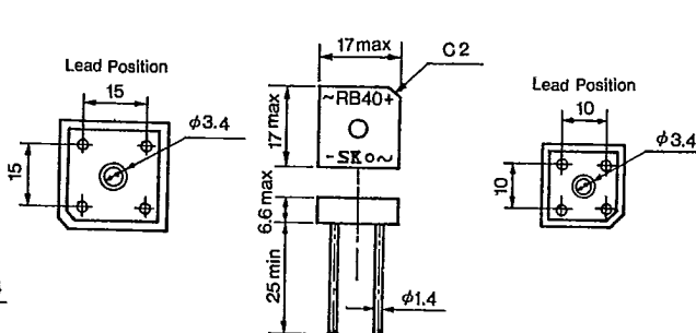
Outline Drawing ②4
