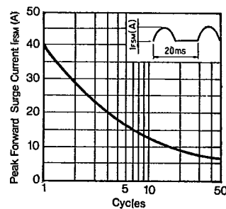
IFSM Characteristics
