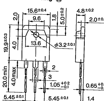
Outline Drawing ②0
