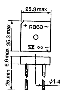
Outline Drawing 23
