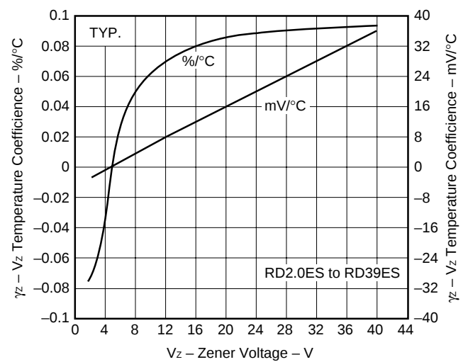
Fig. 9 ZENER VOLTAGE TEMPERATURE COEFFICIENT vs. ZENER VOLTAGE
