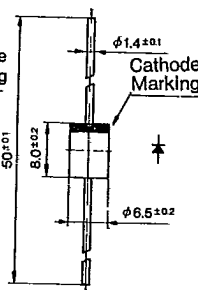
Outline Drawing 84
