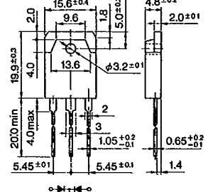
Outline Drawing 84
