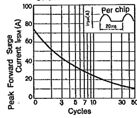
I_{FSM} Characteristics
