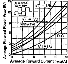
P_F(I_F) - I_F Characteristics
