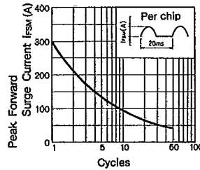
I_{FSM} Characteristics
