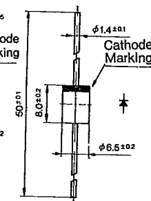
Outline Drawing ⑧⑤
