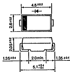
Outline Drawing ⑧①
