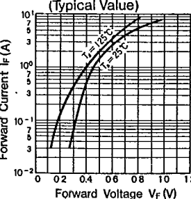
IF-VF Characteristics (Typical Value)
