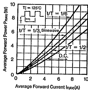
P_F(I_F) - I_F Characteristics
