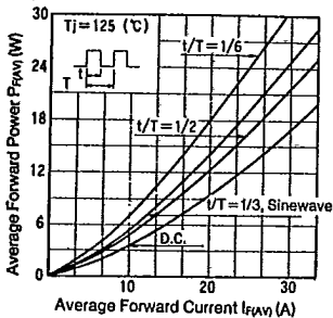
P_F(I_F) - I_F Characteristics
