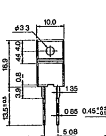
Outline Drawing ⑧①
