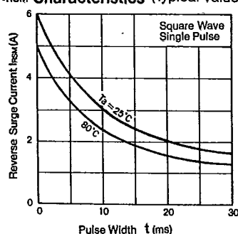
I_{RSM} Characteristics (Typical Value)
