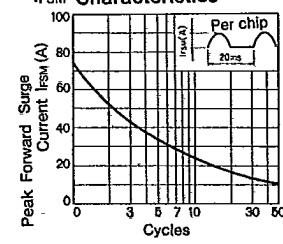
I_{FSM} Characteristics
