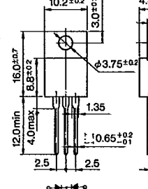
Outline Drawing ⑧④
