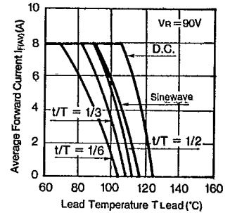
I_F(I_F) - T_{Lead} Characteristics
