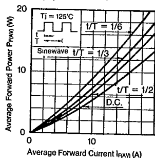
P_F(I_F) - I_F Characteristics
