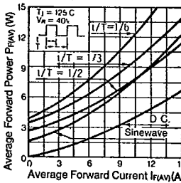
P_F(I_F) - I_F Characteristics
