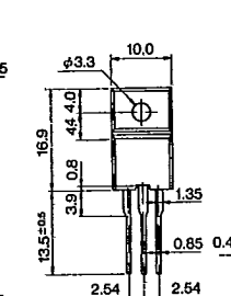
Outline Drawing ⑧②
