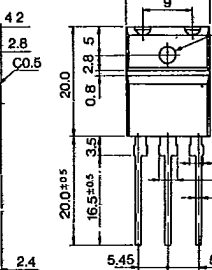
Outline Drawing ⑧③
