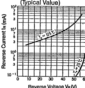
IR - VR Characteristics (Typical Value)
