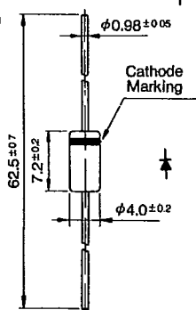
Outline Drawing 59
