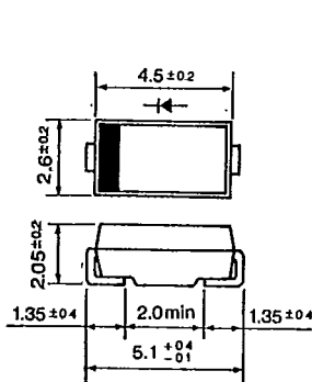
Outline Drawing 59
