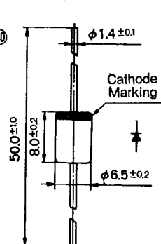
Outline Drawing 60
