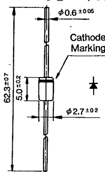
Outline Drawing 56
