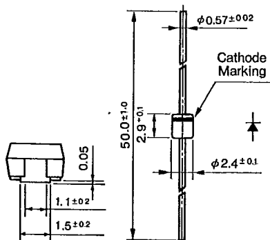
Outline Drawing 60
