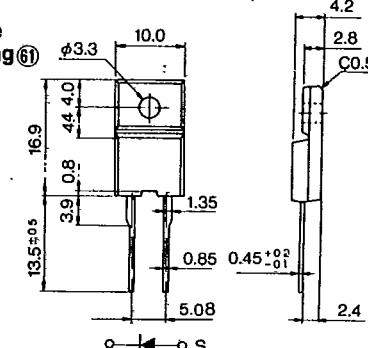
Outline Drawing 61
