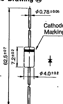
Outline Drawing 58
