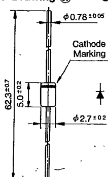
Outline Drawing 61
