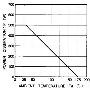
Fig. 4 Derating curve
