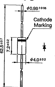
Outline Drawing ⑥
