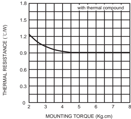
CONTACT THERMAL RESISTANCE r_{cf}
