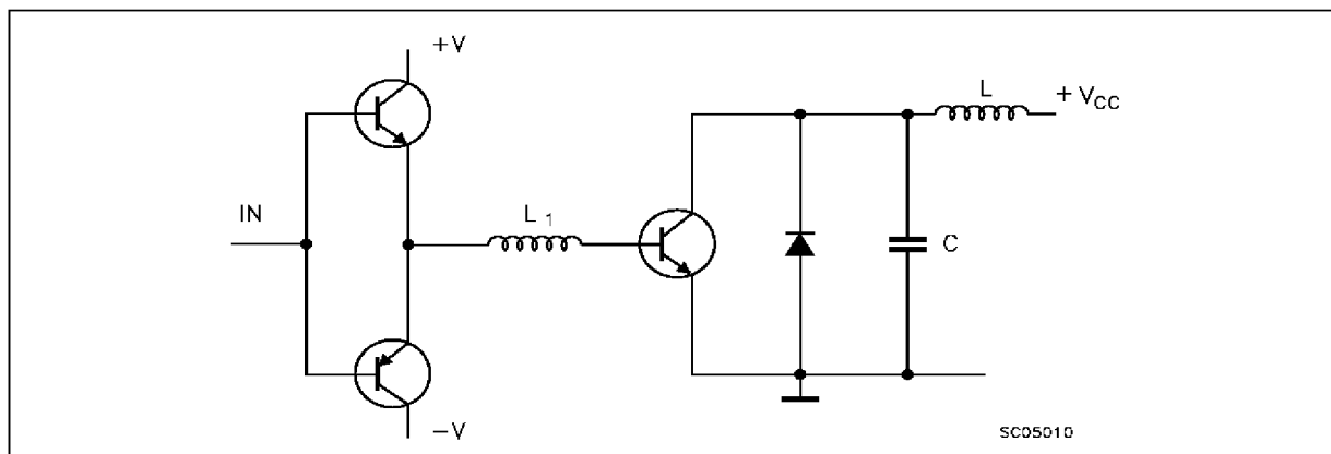
Figure 1: Inductive Load Switching Test Circuit.
