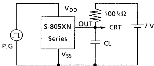
(5) Dynamic response characteristics
