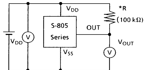
(6) Minimum operating voltage
