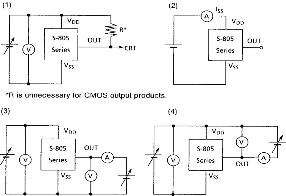
Figure 6 Test circuit
