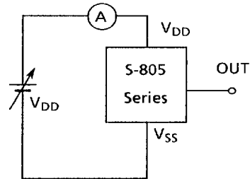
(6) Minimum operating voltage
