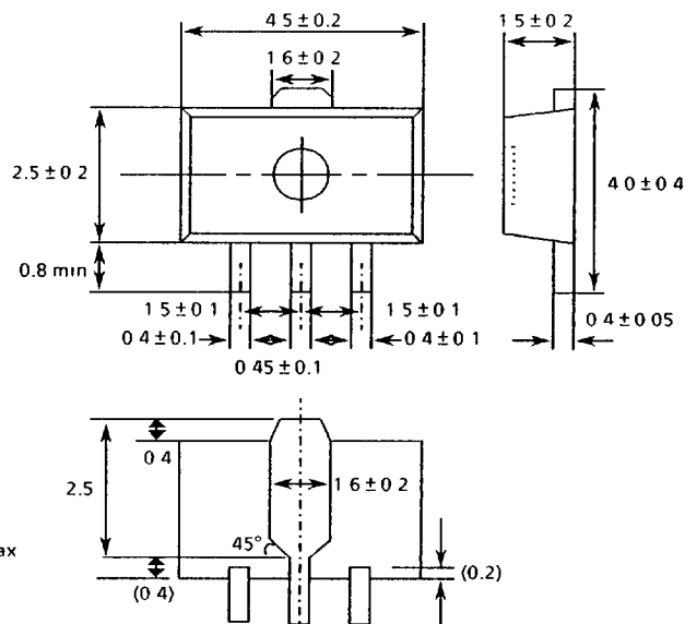
Figure 7 Dimensions
