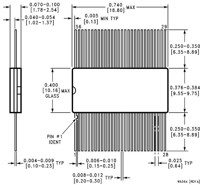
56-Lead Ceramic Flatpak (F) Order Number SCAN182245AFMQB Package Number WA56A
