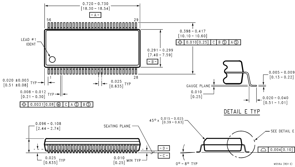
56-Lead SSOP (0.300" Wide) (SS) Order Number SCAN182245ASSC or SCAN182245ASSCX Package Number MS56A
