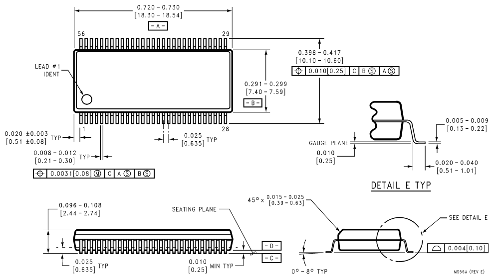
56-Lead SSOP (0.300" Wide) (SS) Order Number SCAN182373ASSC or SCAN182373ASSCX Package Number MS56A
