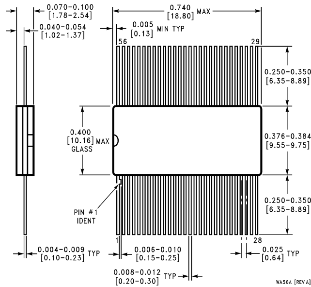
56-Lead Ceramic Flatpak (F) Order Number SCAN182373AFMQB Package Number WA56A
