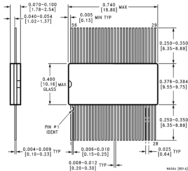
56-Lead Ceramic Flatpak (F) Order Number SCAN18373TFMQB Package Number WA56A
