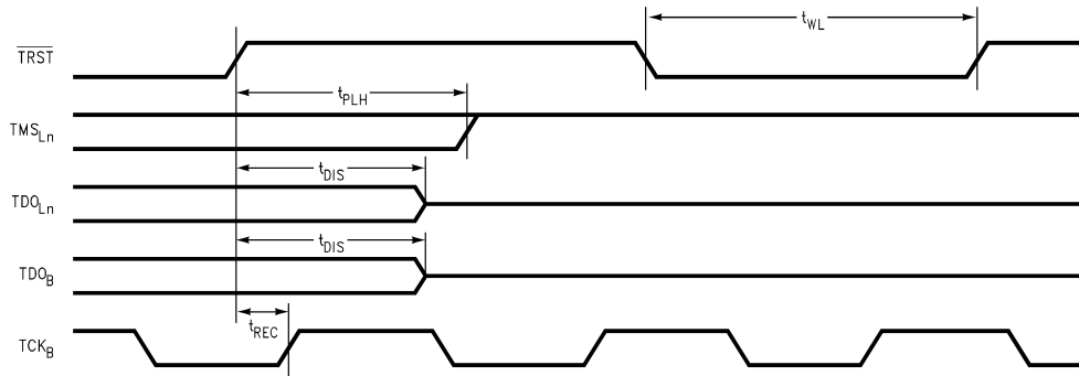
FIGURE 15. Reset Waveforms
