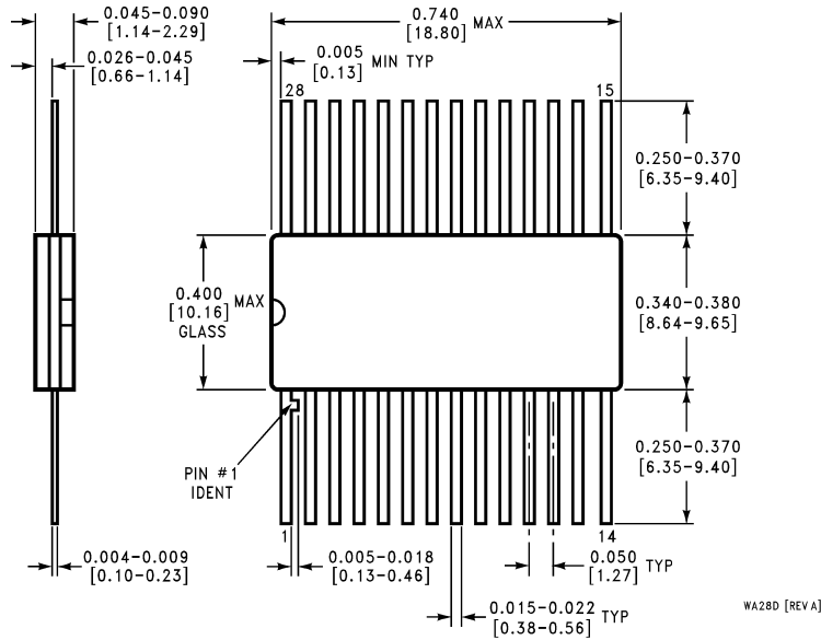
28-Pin Flatpak Package Number WA28D
