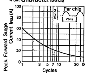
I_{FSM} Characteristics
