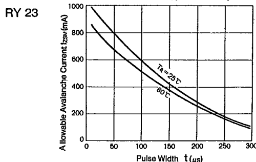
I_{ZSM} Characteristics (Typical Value)
