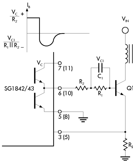
FIGURE 17. — BIPOLAR TRANSISTOR DRIVE
