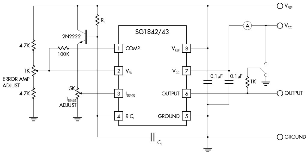
FIGURE 24. — OPEN LOOP LABORATORY FIXTURE
