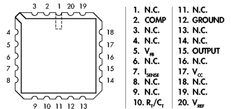
I PACKAGE (Top View)
