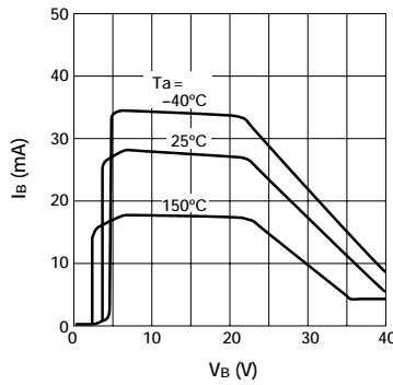
■ Circuit Current
