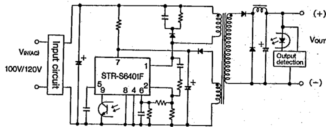
Forward converter
