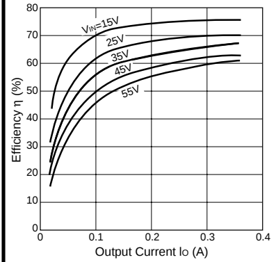
Efficiency Characteristics
