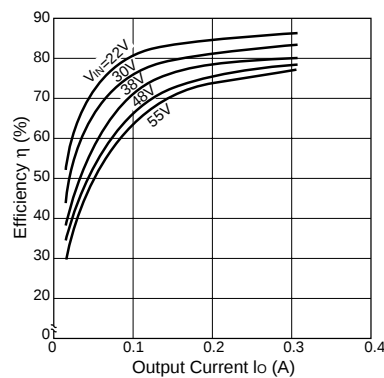
Efficiency Characteristics
