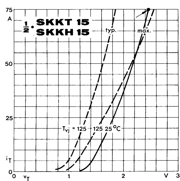
Fig. 8 On-state characteristics
