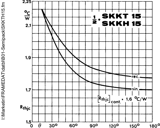
Fig. 7 Thermal resistance vs. conduction angle
