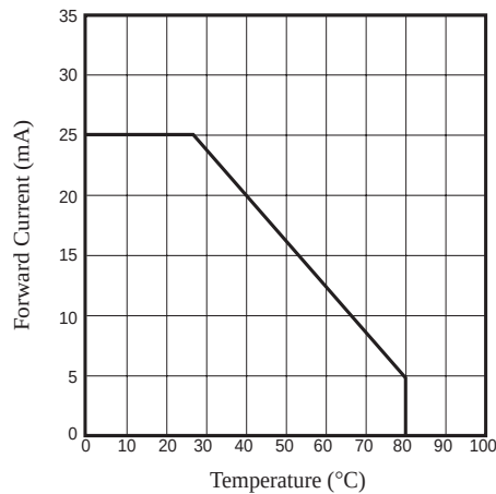
Forward Current Derating (Absolute Maximum Rating)
