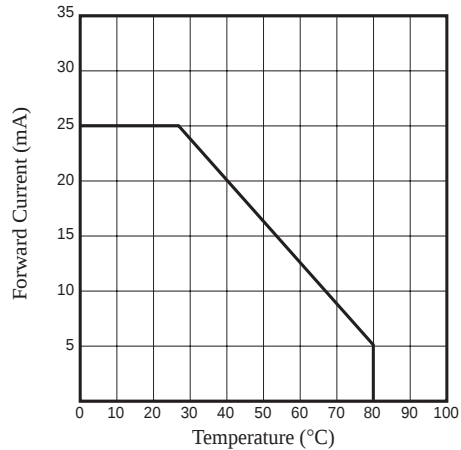
Forward Current Derating (Abbsolute Maximum Rating)
