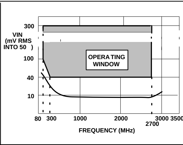
Fig. 5b Typical input sensitivity (Prescaler enabled, DE=1)
