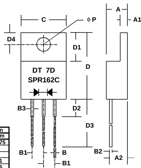
TO - 220AB
