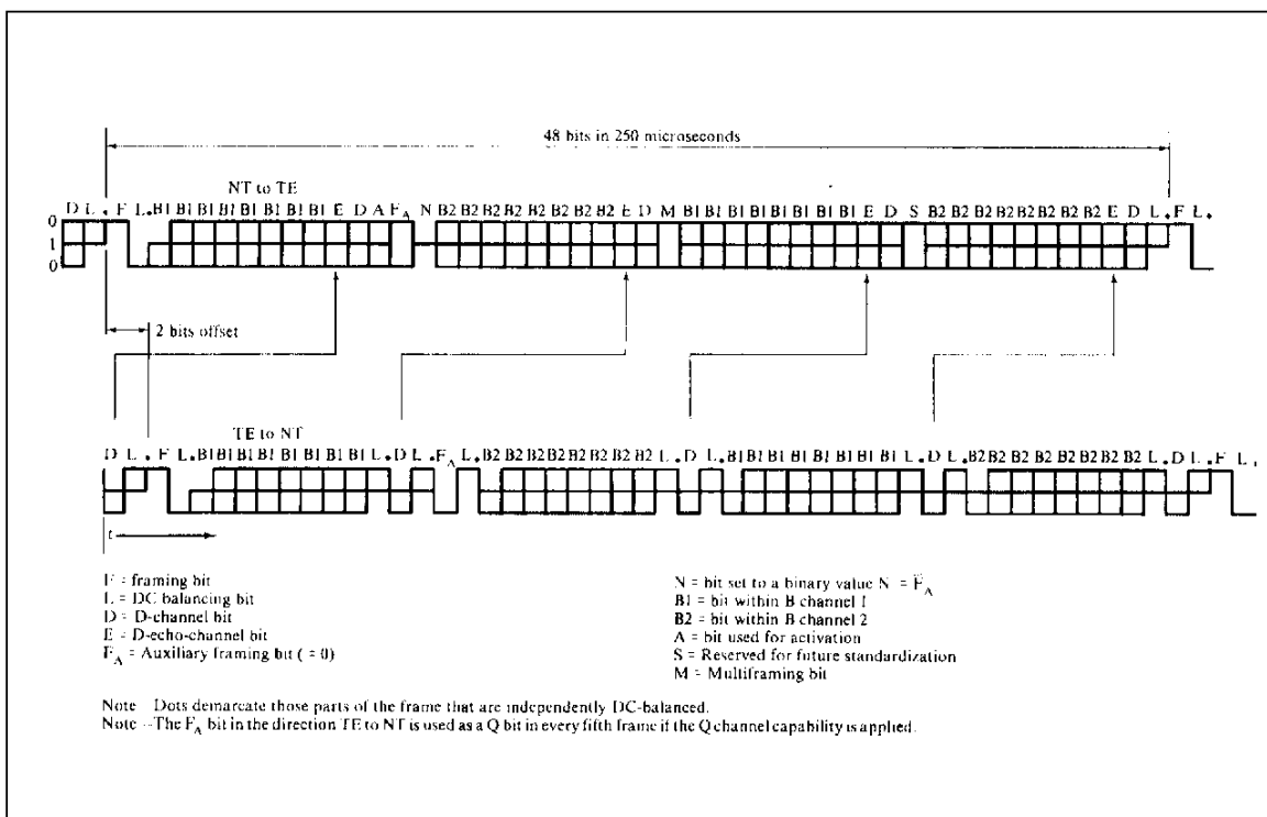
Figure 2: Frame Format
