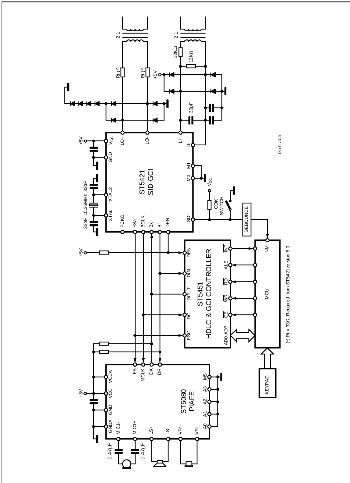
Figure 7: ISDN Telephone Set Application (non isolated)
