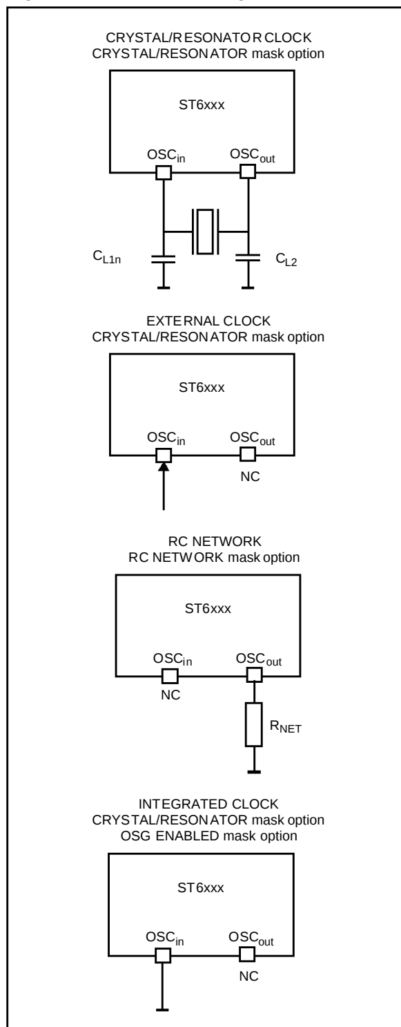
Figure 11. Oscillator Configurations
