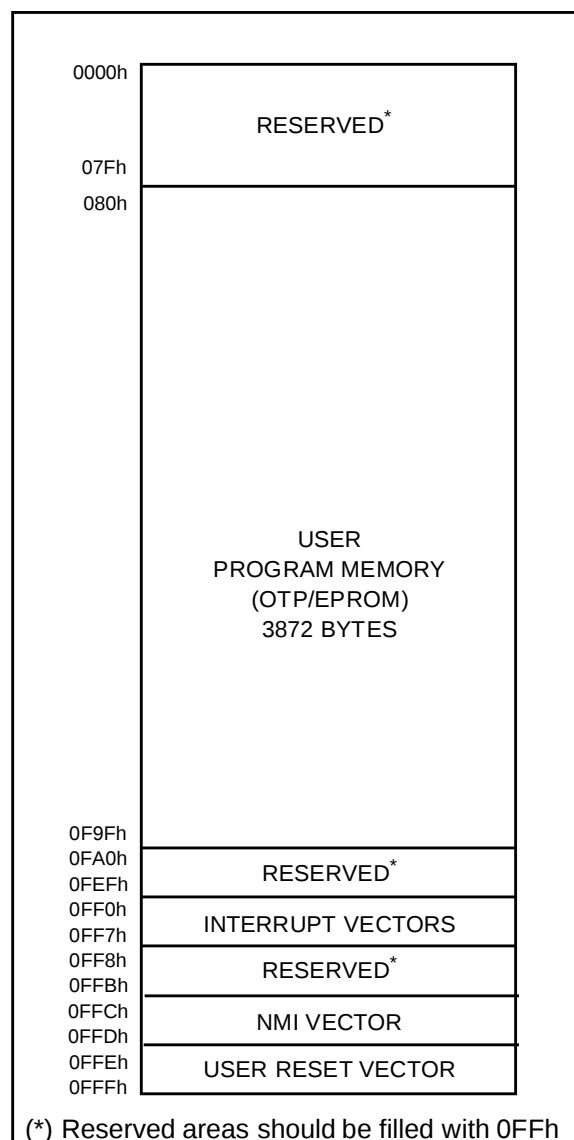
Figure 5. ST62T20, T25, E20, E25 Program Memory Map
