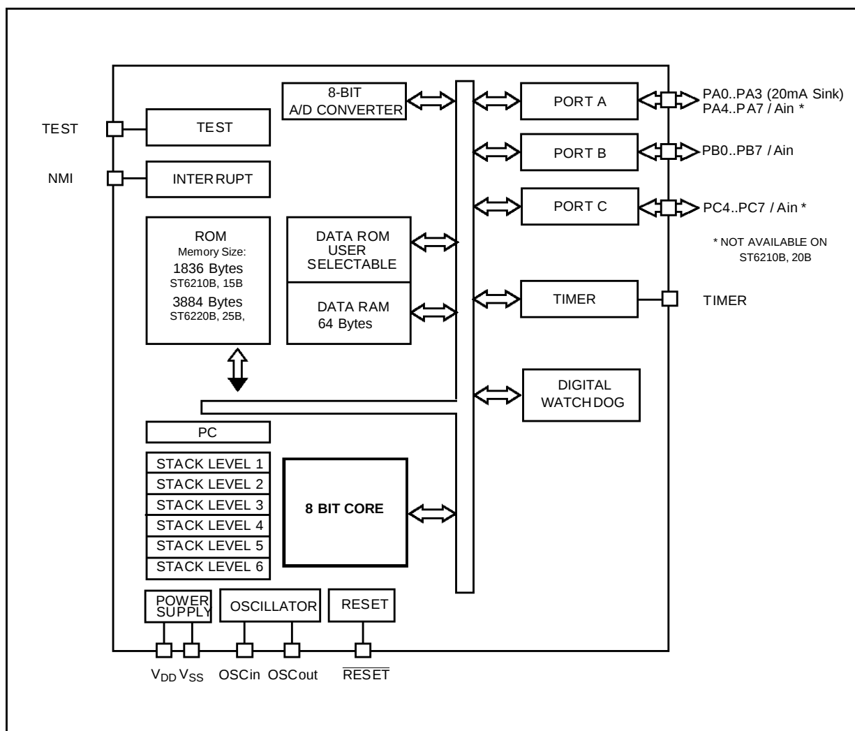
Figure 2. Block Diagram
