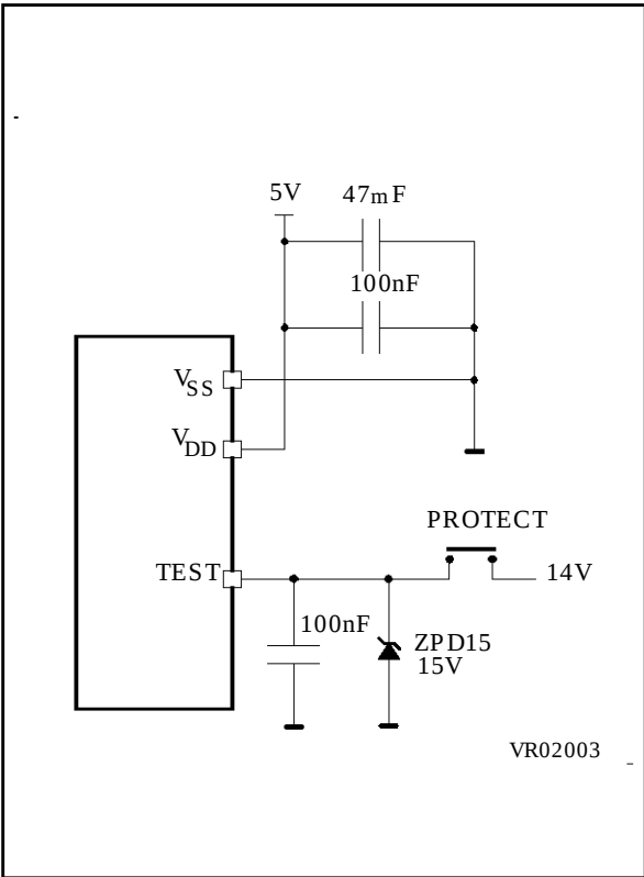
Figure 34. Programming Circuit
