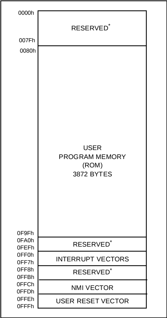
Figure 7. ST6220B/25B Program Memory Map
