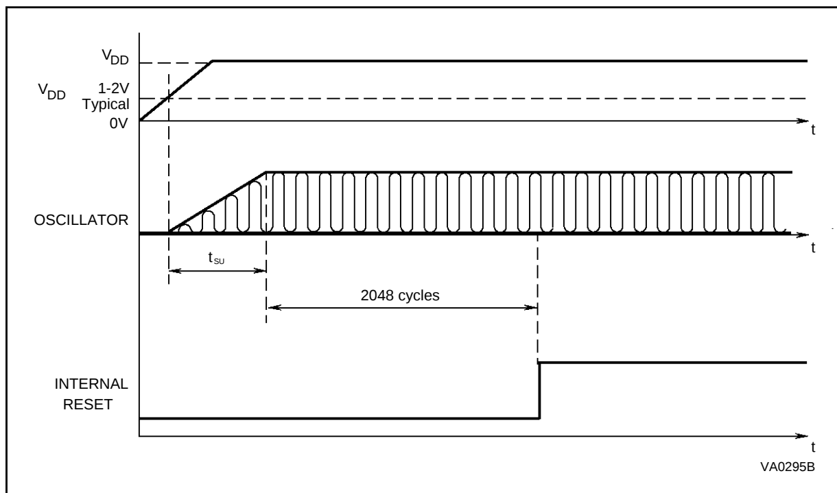
Figure 30. Power-on-Reset
