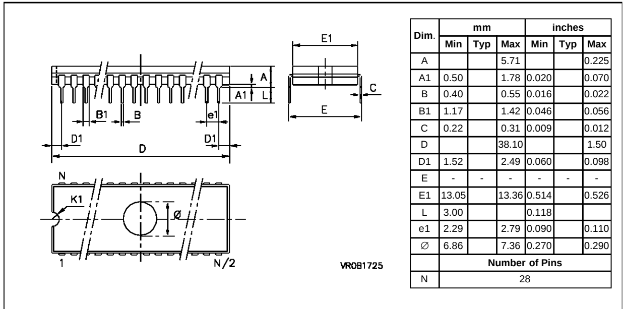
Figure 11. 28-Ceramic Dual In Line Package, 600-mil Width
