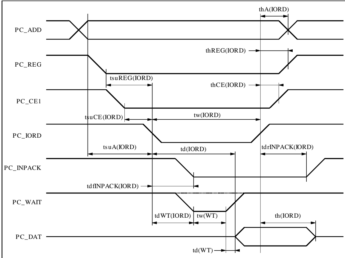
Figure 15 : Read Timing Diagram
