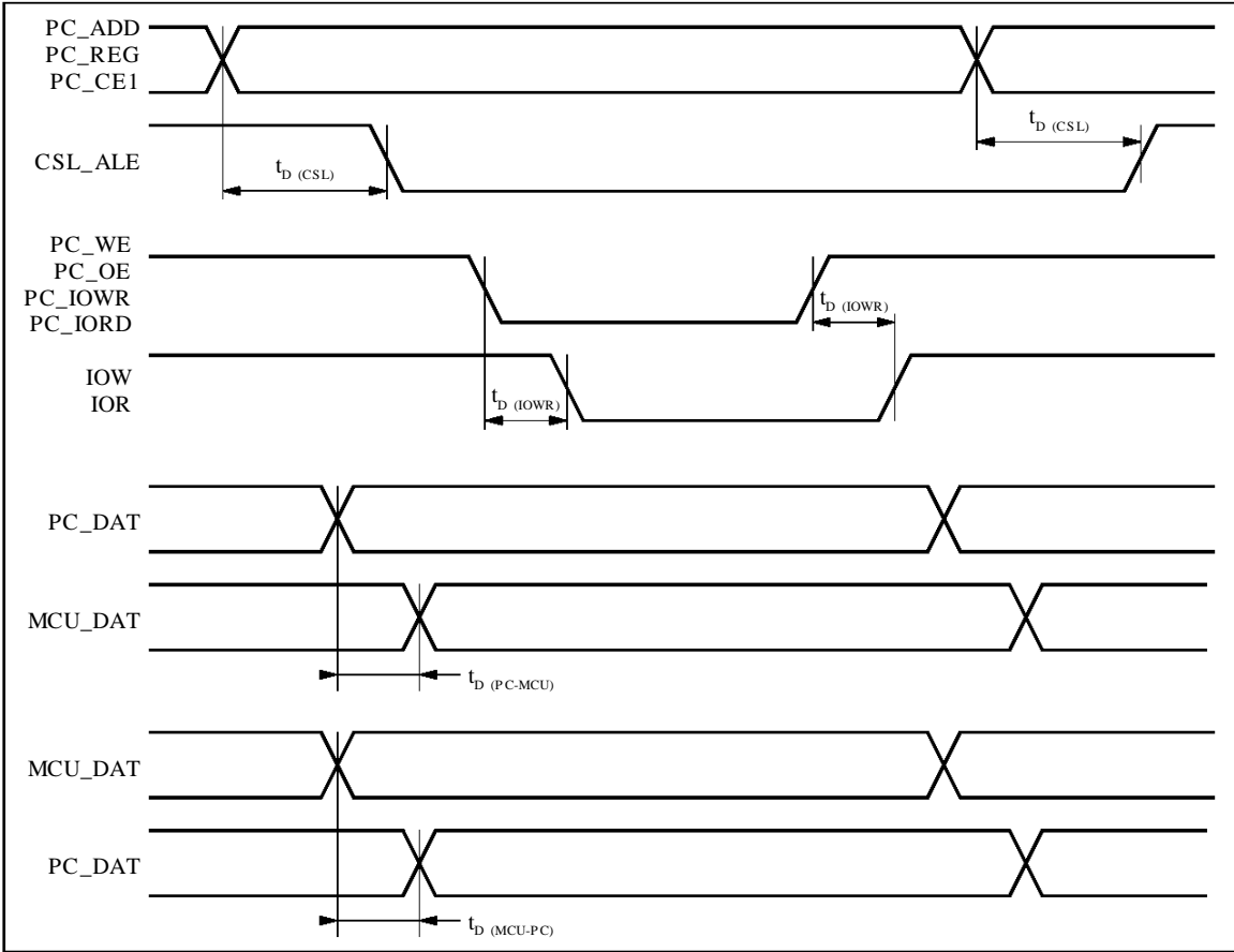
Figure 21 : Transfer Timing Diagram
