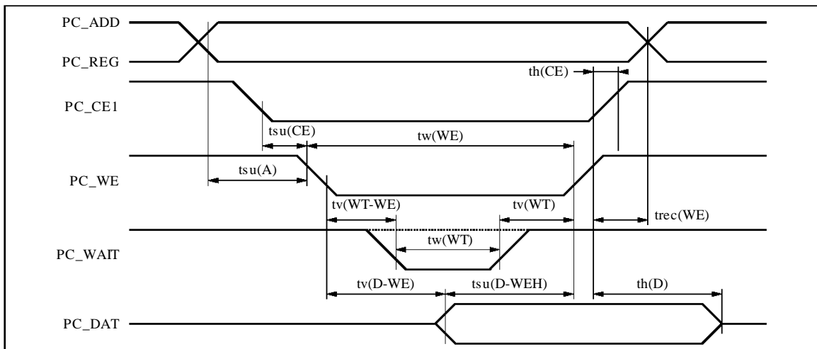
Figure 12 : Write Timing Diagram
