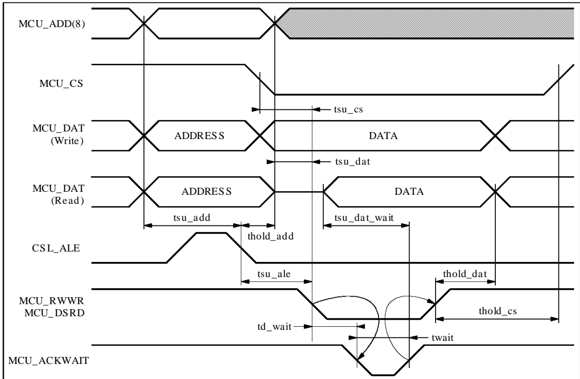
Figure 20 : MCU_MOTEL is Tied to '0'
