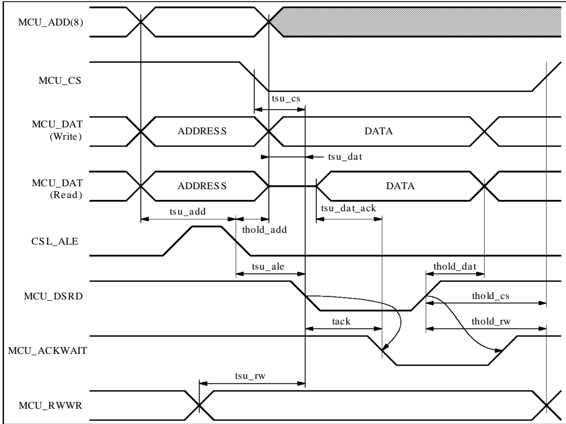
Figure 19 : MCU_MOTEL is Tied to '1'
