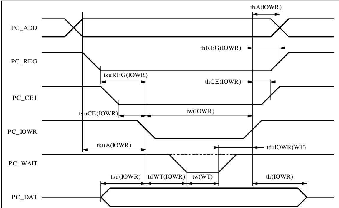
Figure 16 : Write Timing Diagram
