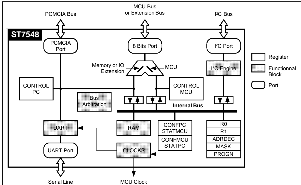
Figure 2 : Chip Block Diagram
