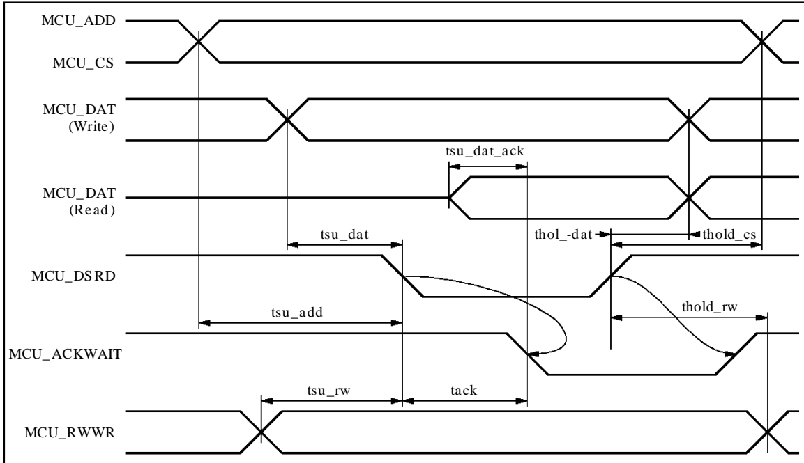
Figure 17 : MCU_MOTEL is Tied to '1'
