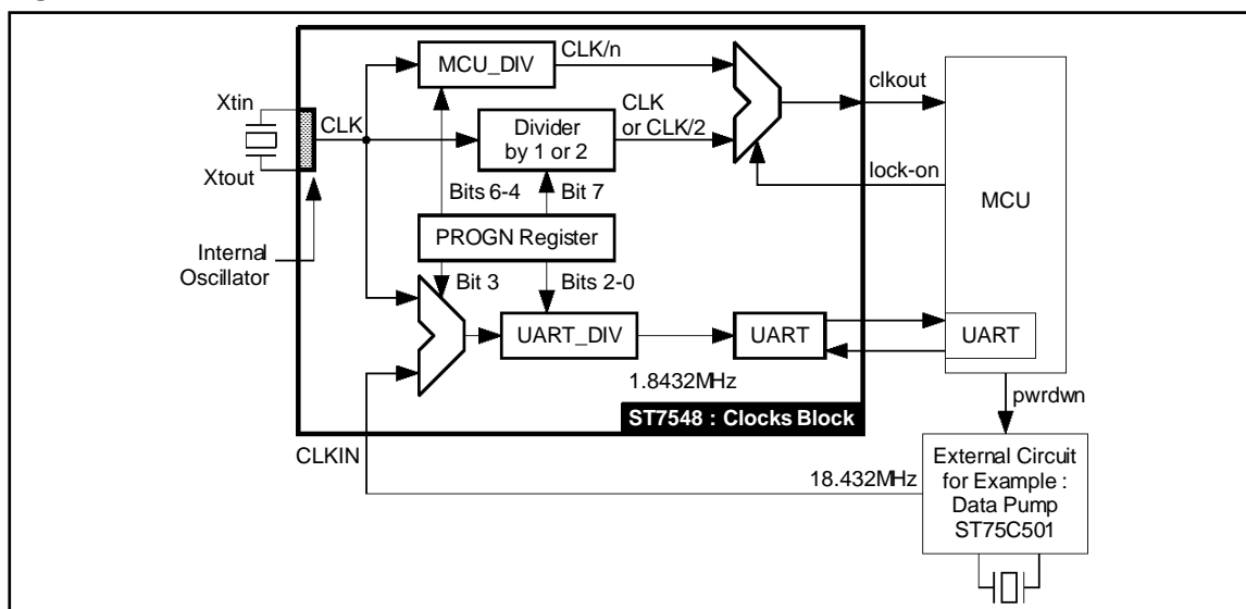
Figure 3 : Theoretical Schematic
