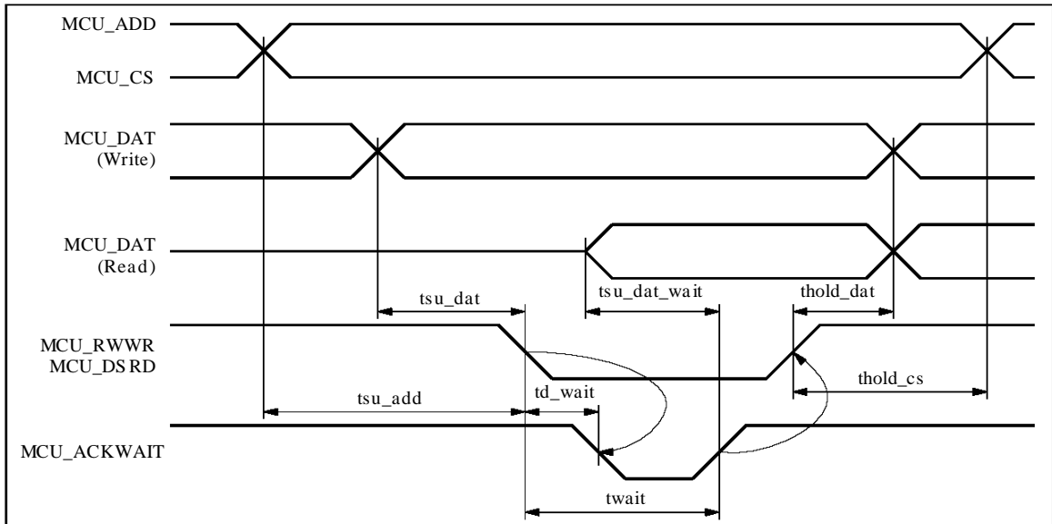
Figure 18 : MCU_MOTEL is Tied to '0'
