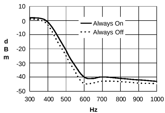
Figure D2 : Call Progress Tone Detector Band 1
