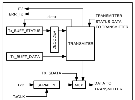
Figure H2 : Tx Buffer Schematics
