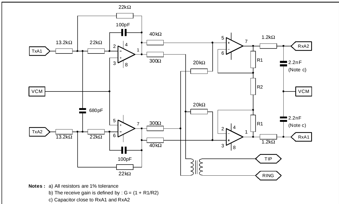
Figure F1 : Typical line interface
