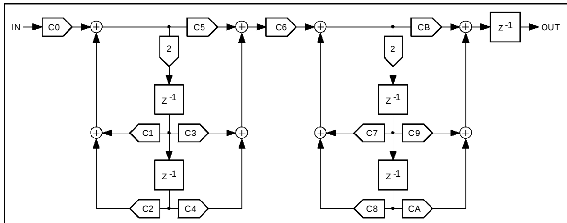
Figure G1 : Biquadratic IIR Filter
