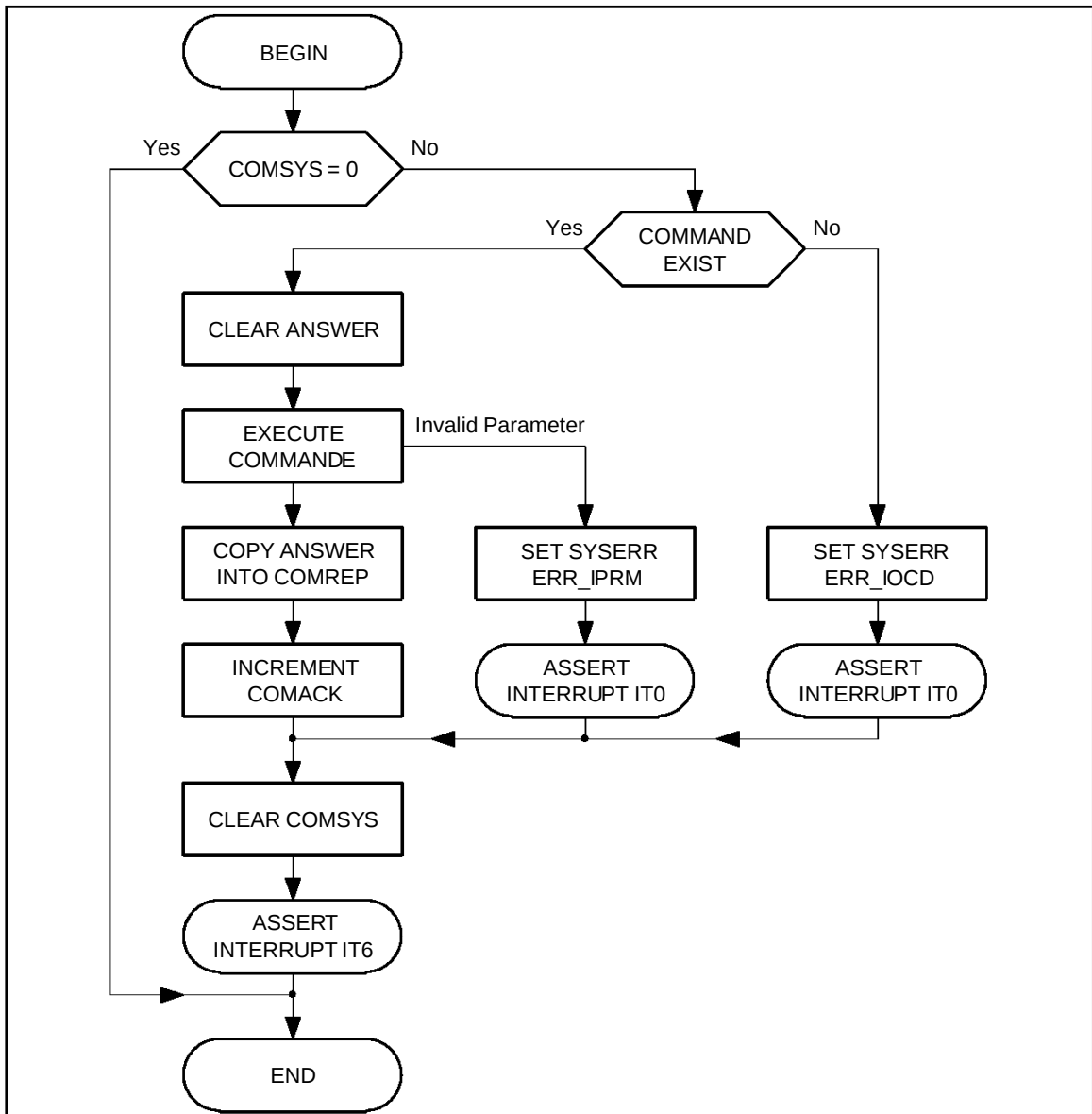
Figure B1 : Command Acknowledge
