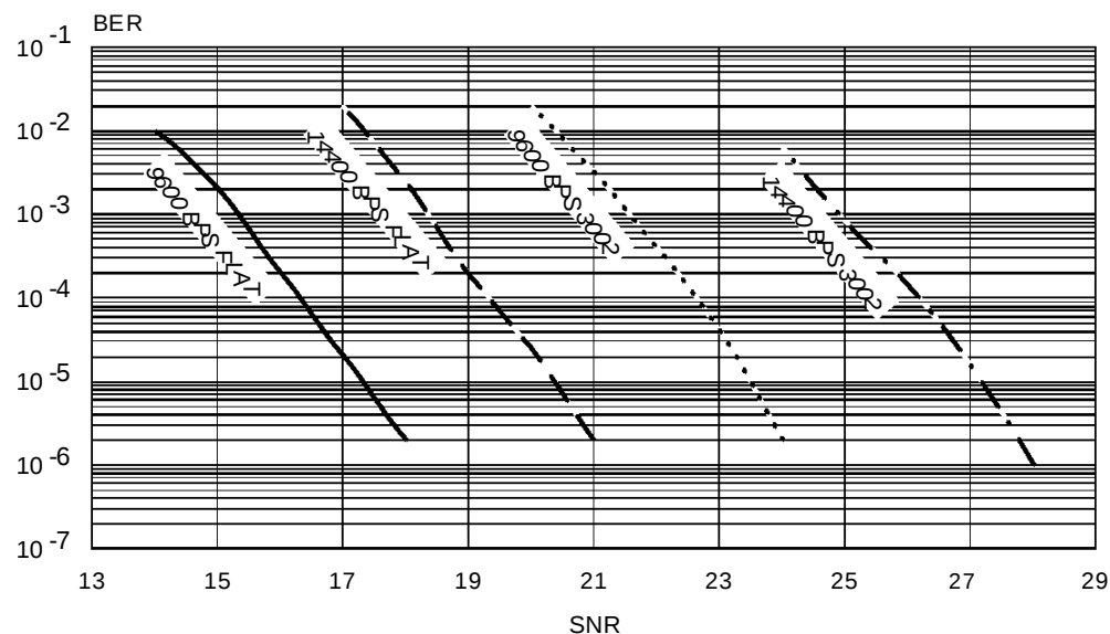
Figure C1 : Typical V32bis BER performances
