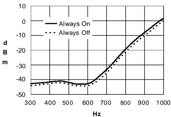
Figure D1 : Call Progress Tone Detector Band 0
