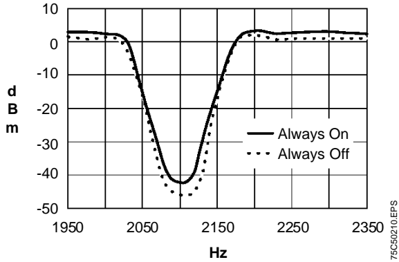
Figure E1 : 2100Hz Answer Tone Detector
