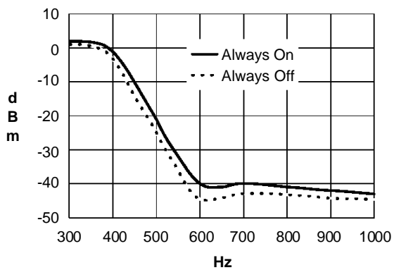
Figure D2 : Call Progress Tone Detector Band 1
