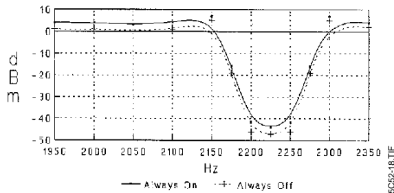
Figure 13 : 2225Hz Answer Tone Detector
