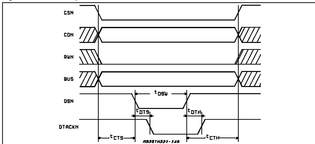
Figure 14: CPU Read Cycle
