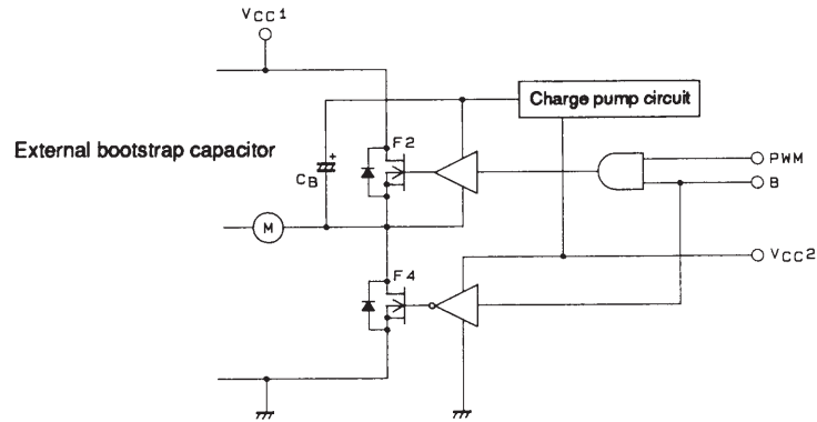
Figure 7 Upper and Lower MOSFET Drive Circuits
