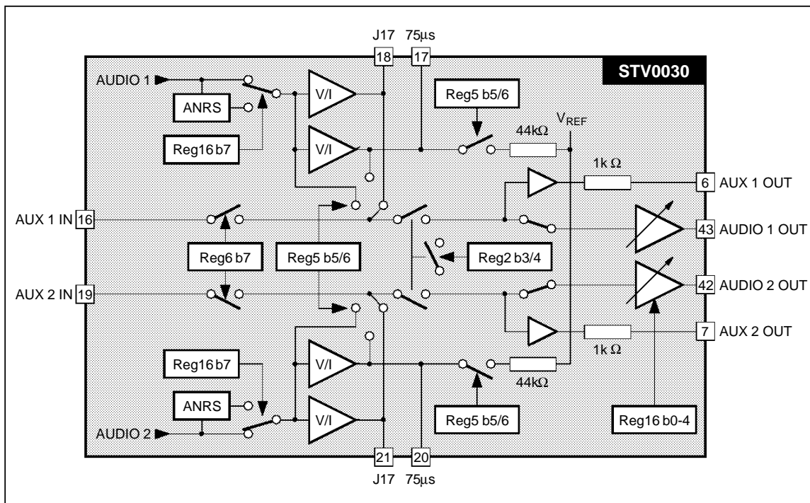
Figure 4 : Audio Processing Block Diagram
