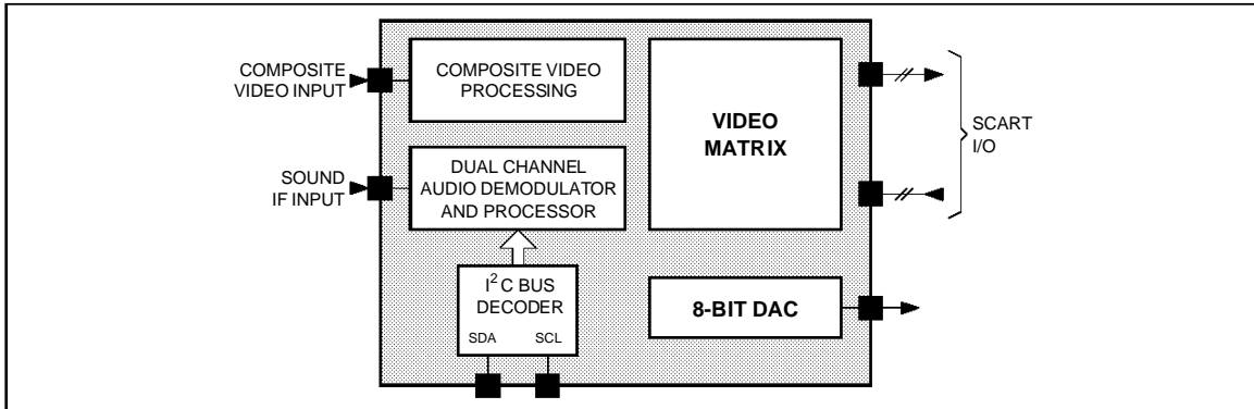
Figure 2 : Video Processing Block Diagram
