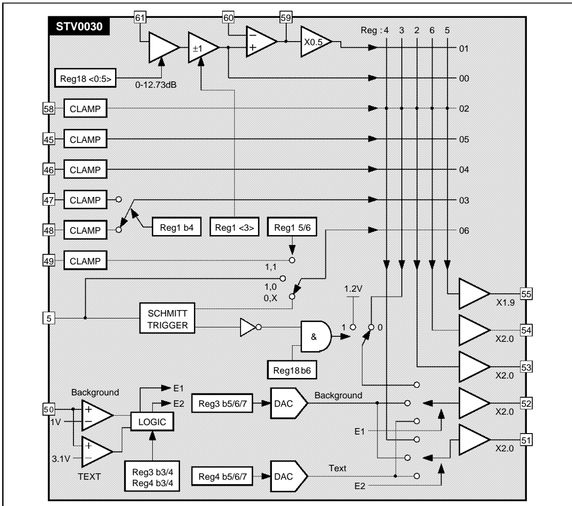
Figure 2 : Video Processing Block Diagram
