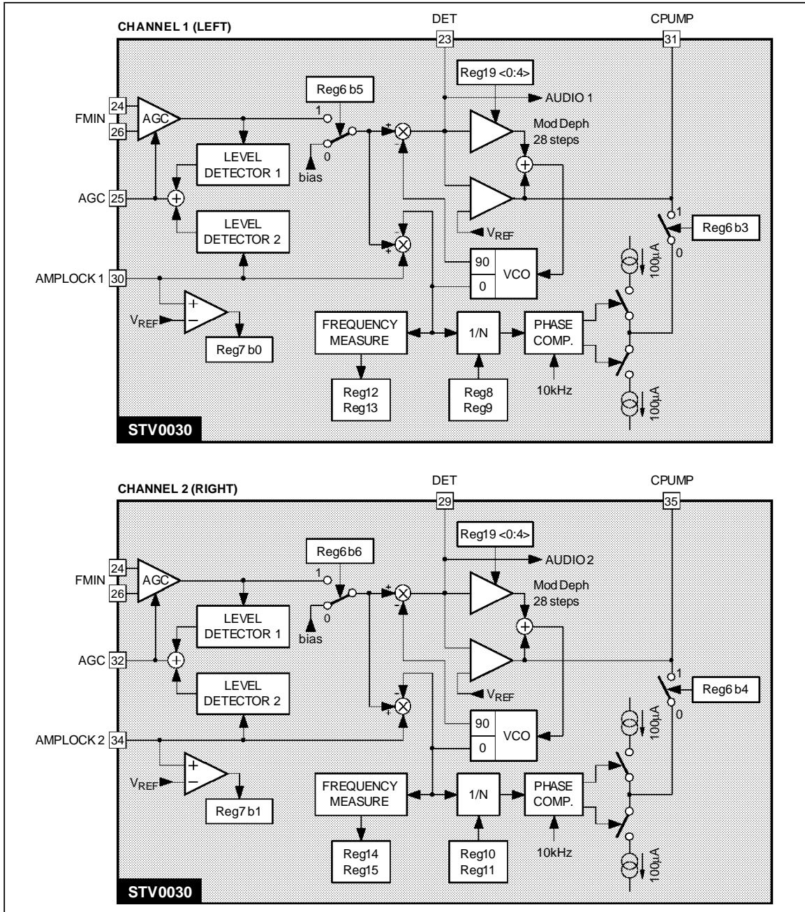
Figure 3 : FM Demodulation Block Diagram
