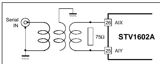
Figure 12 : Equalizer Transformer Input Circuit
