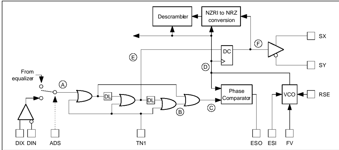
Figure 18 : x^9 + x^4 + 1 Descrambler
