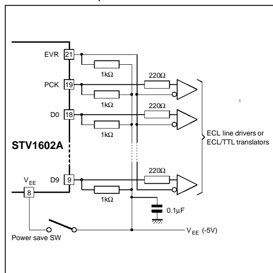
Figure 2 : A Suggested Parallel Clock / Data Output Circuit
