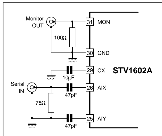
Figure 11 : Equalizer Capacitor Coupling Input Circuit
