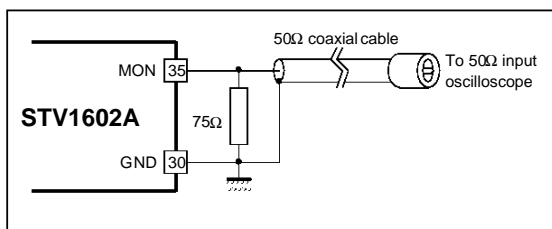
Figure 14 : Equalized Waveforms Monitoring
