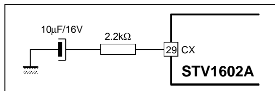
Figure 15 : AGC Time Constant
