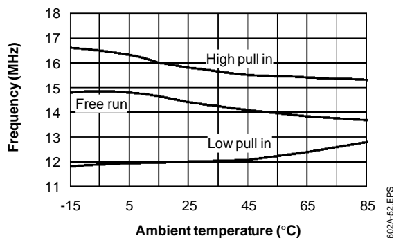
Figure 34 : Pull-in Range and Free Run Frequency (143Mb/s)
