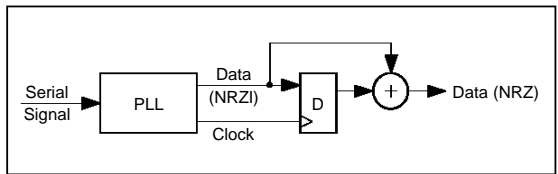
Figure 17 : NRZI to NRZ conversion
