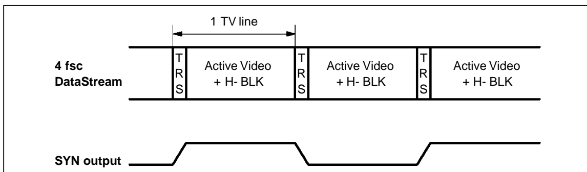
Figure 21 : SYNC Output in 4 fsc Case (not to scale)
