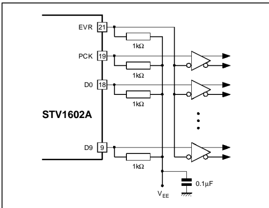
Figure 24 : A Circuit Example to Disable Parallel Clock
