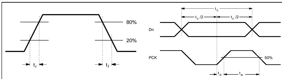
Figure 1 : t_r , t_f , t_c , t_d Definition
