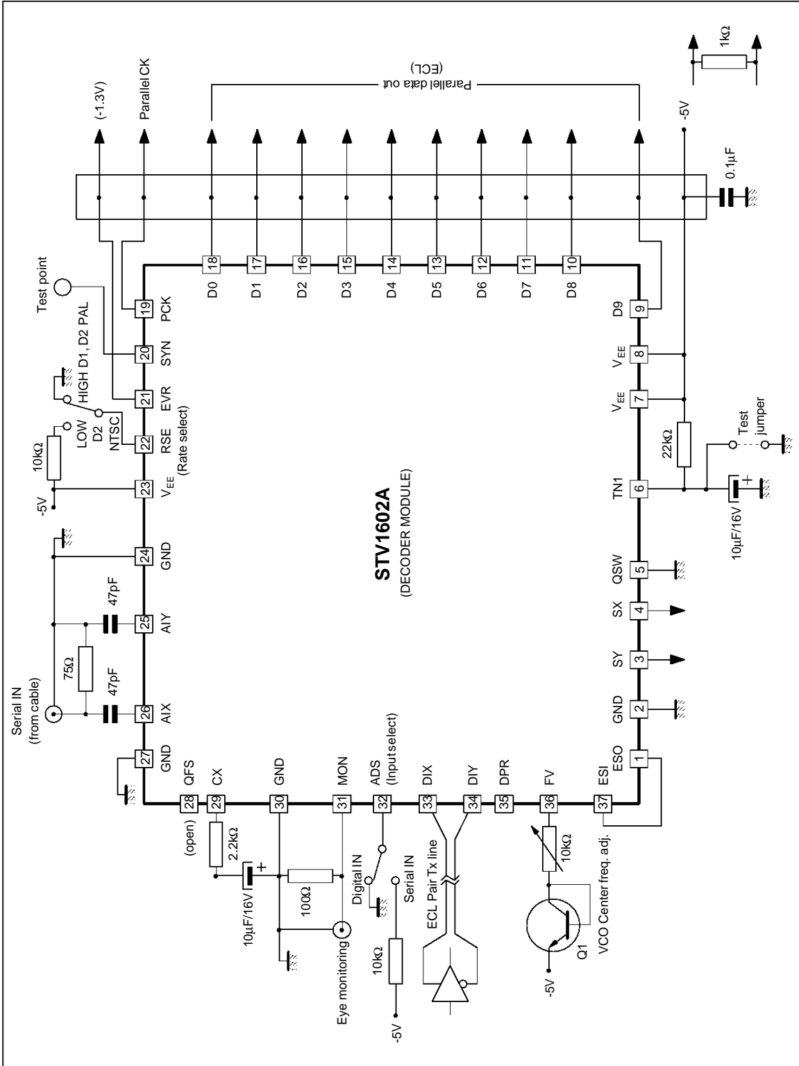
Figure 28 : Application Circuit Example
