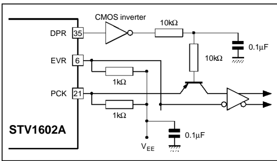
Figure 24 : A Circuit Example to Disable Parallel Clock
