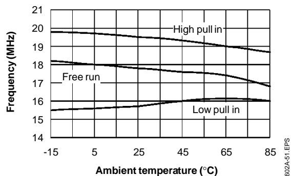
Figure 33 : Pull-in Range and Free Run Frequency (177Mb/s)
