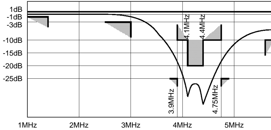
Figure 1 : SECAM Trap Filter Frequency Response (Maximum group delay time at 3.9MHz : 240ns (typical 220ns))
