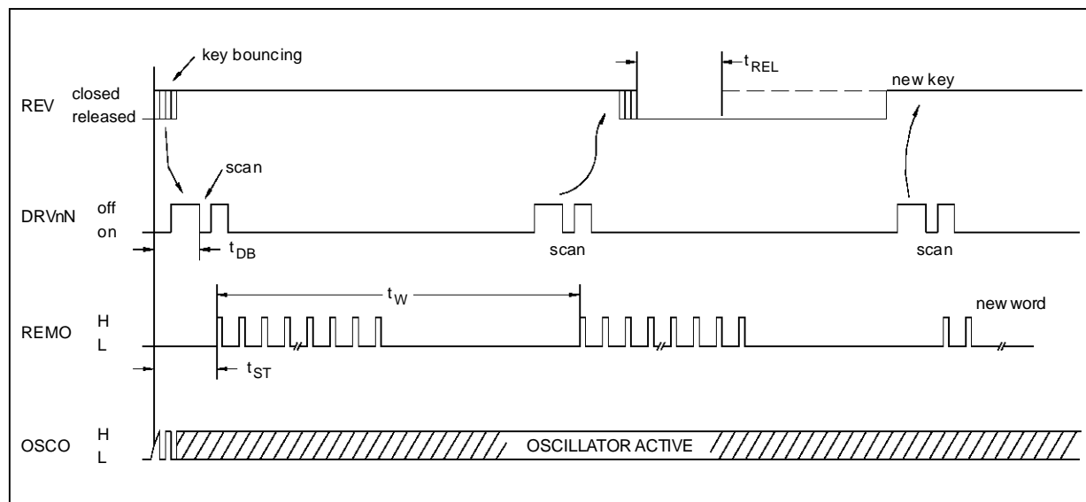
Figure 3 : Single Key-stroke Sequence. Debounce time : t DB = 4 to 9 x t 0 , Start time : t ST = 5 to 10 x t 0 , Minimum release time : t REL = t 0 .
