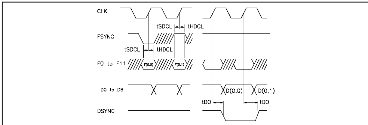
Synchronization Signals Timing Diagram for an Inverse Transform
