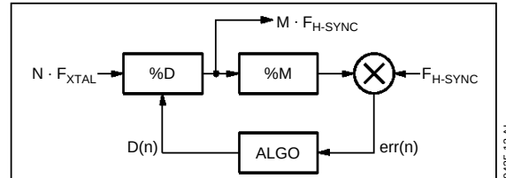
Figure 10 : Digital PLL
