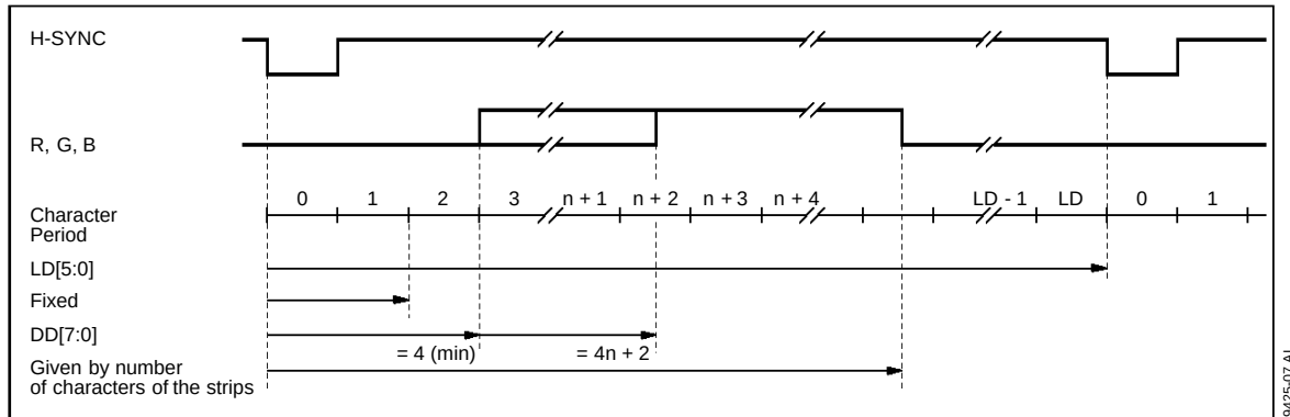
Figure 5 : Horizontal Timing
