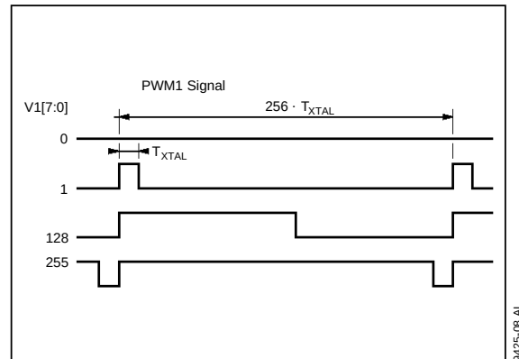
Figure 6 : PWM Timing
