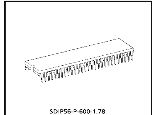
SDIP56-P-600-1.78
