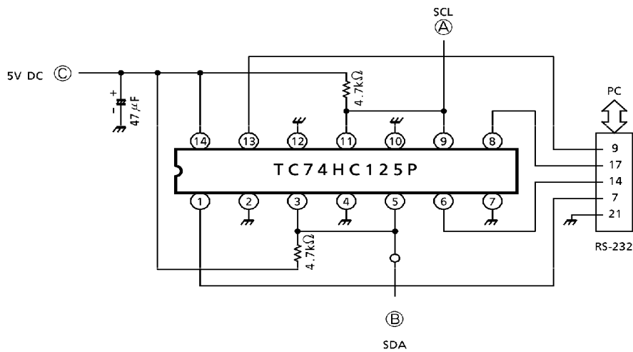
I 2 C BUS Interface
