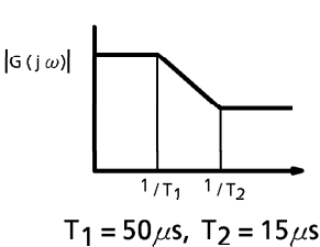
Fig.6 Filter characteristic
