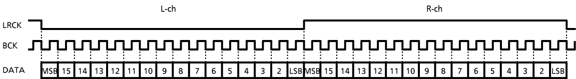
Fig.2 Example of input timing chart (When R/L=M/L="H")
