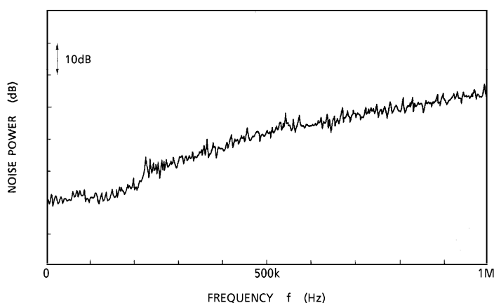
Fig.8 Noise shaping characteristic
