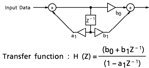
Fig.5 Construction of IIR type digital De-emphasis Filter
