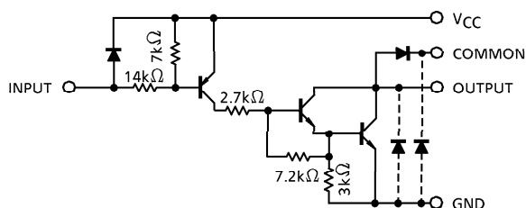
TD62386AP, TD62386AF
