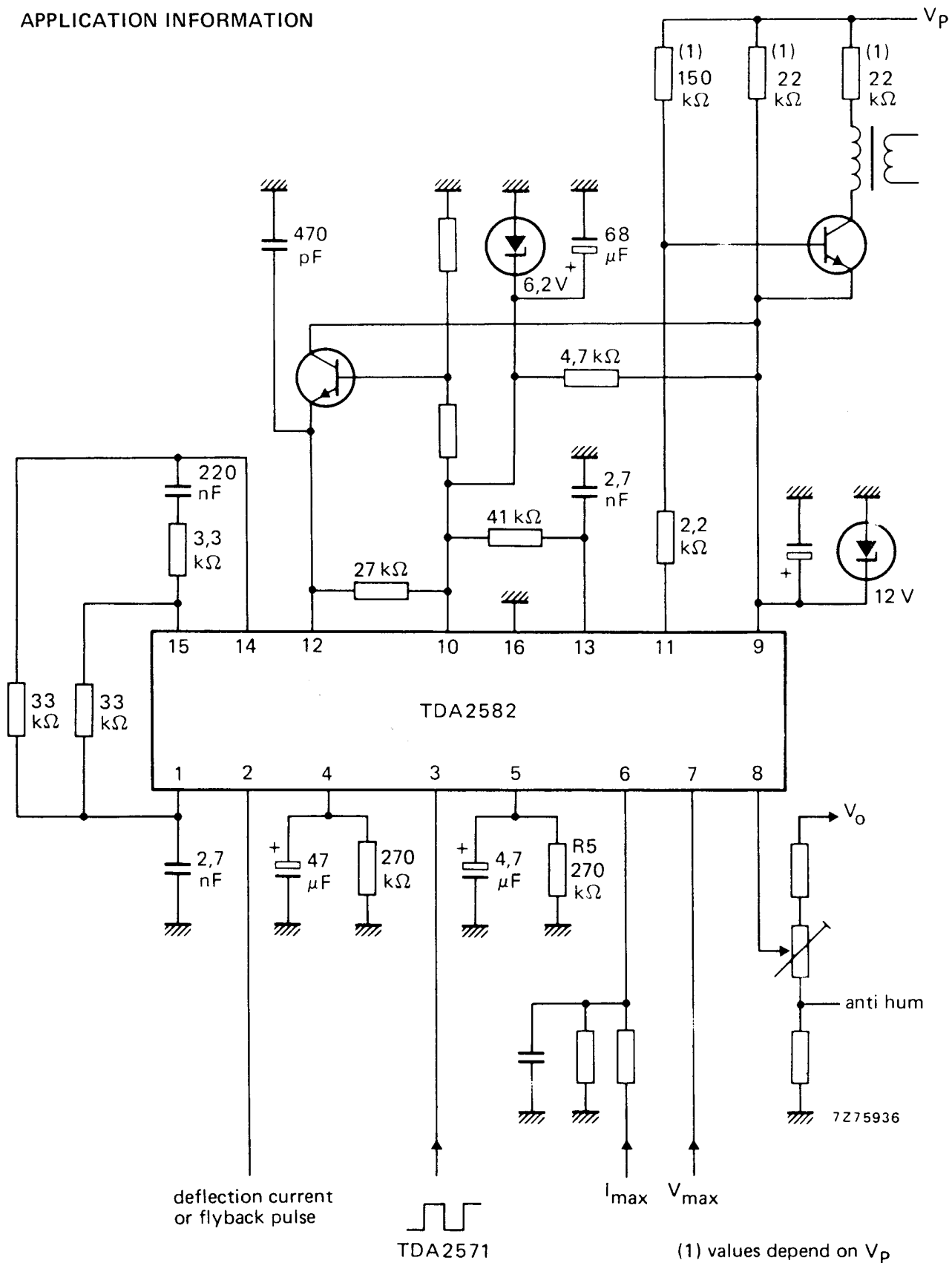
Fig. 4 Circuit diagram.
