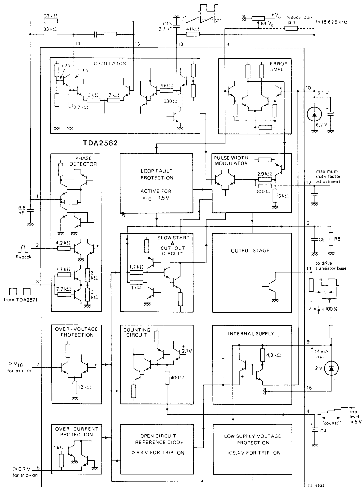
Fig. 1 Block diagram.
