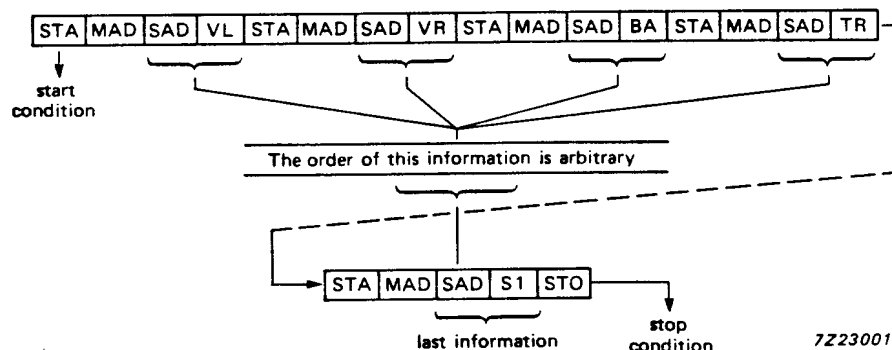
Fig. 4 Data transmission after a power-on reset.
