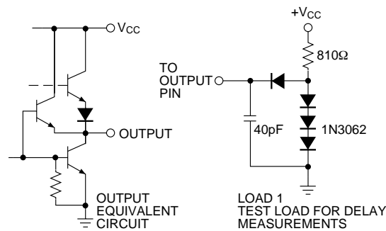
Figure 4. Output Circuits
