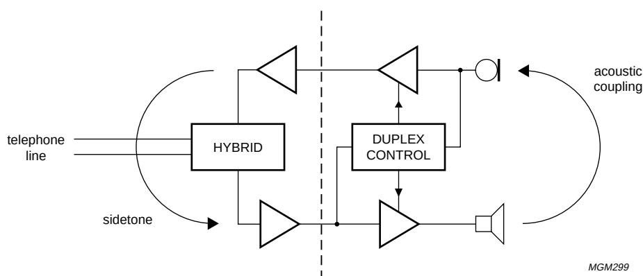
Fig.6 Handsfree telephone set principles.
