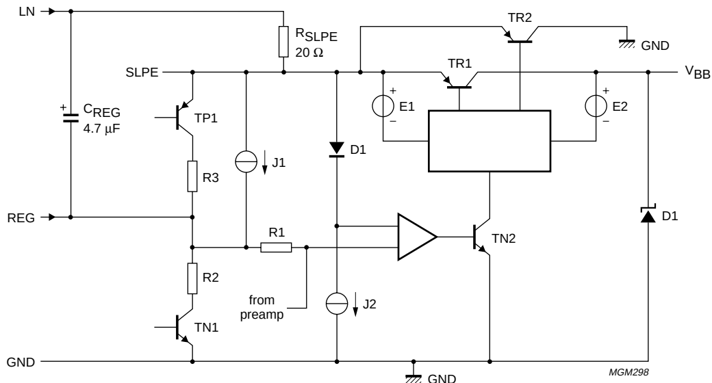
Fig.3 Line interface principle.
