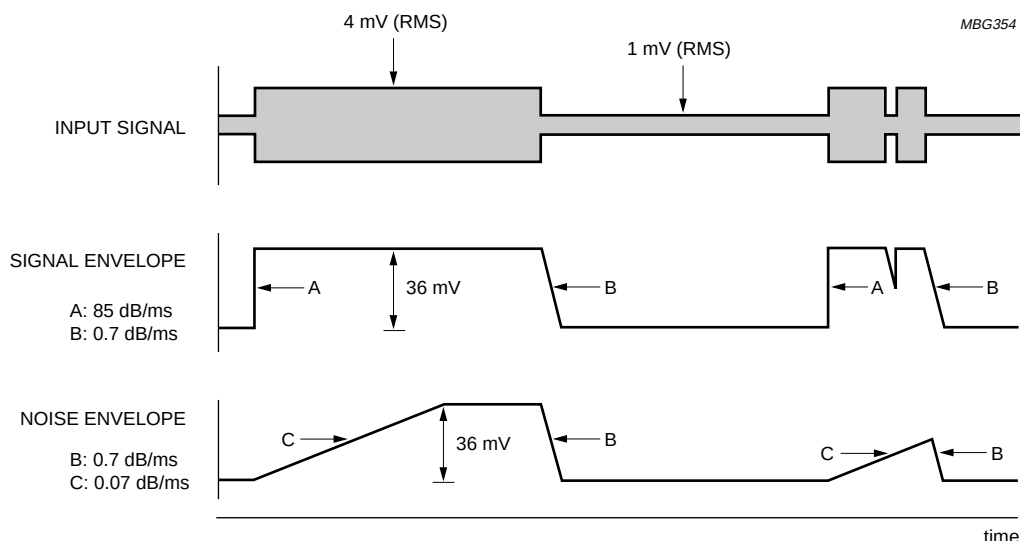
Fig.10 Signal and noise envelope waveforms.
