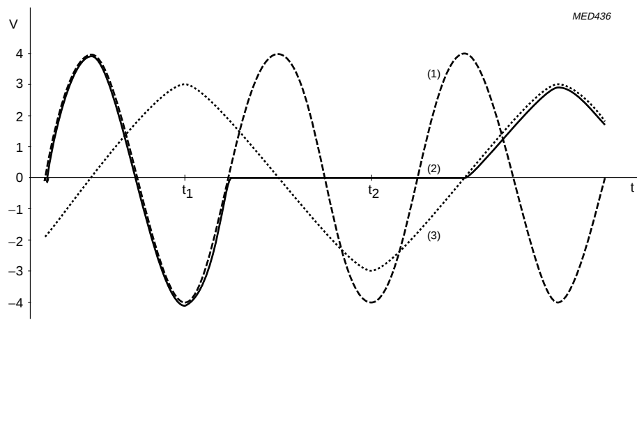
Fig.16 Zero cross function; only one channel shown.
