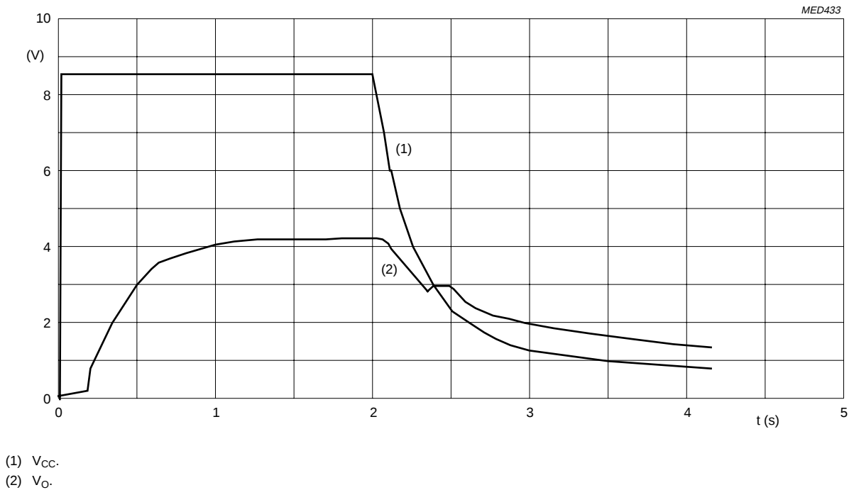
Fig.13 Turn-on/off behaviour.
