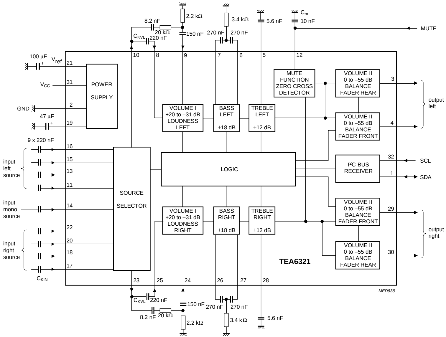
Fig.1 Block diagram.
