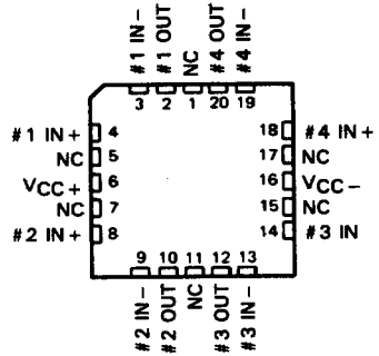
TL084M . . . FK CHIP CARRIER PACKAGE (TOP VIEW)
