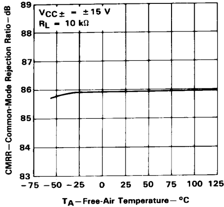
COMMON-MODE REJECTION RATIO vs FREE-AIR TEMPERATURE
