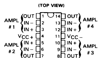
TL084, TL084A, TL084B D, J, OR N PACKAGE
