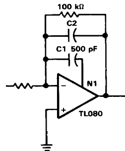
FIGURE 3. FEED-FORWARD COMPENSATION
