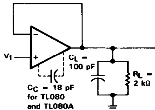
FIGURE 1. UNITY-GAIN AMPLIFIER
