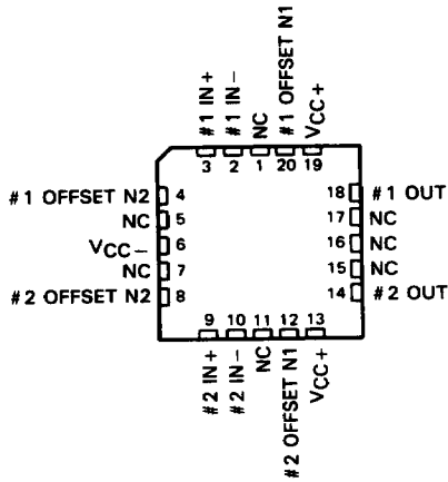
TL083M . . . FK CHIP CARRIER PACKAGE (TOP VIEW)
