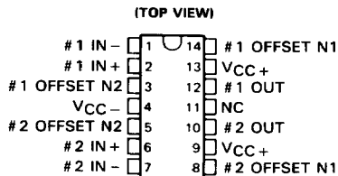
TL083, TL083A D, J, OR N PACKAGE
