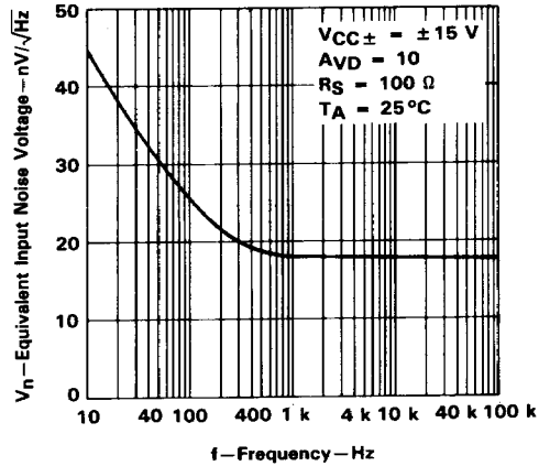
EQUIVALENT INPUT NOISE VOLTAGE vs FREQUENCY
