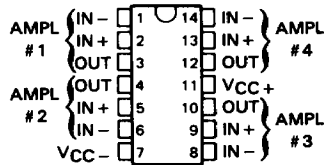
TL085 N PACKAGE (TOP VIEW)
