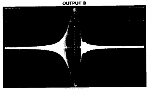
2 kHz/div CASCADED BANDPASS FILTER f_0 = 100 \text{ kHz} , Q = 89 , GAIN = 16
