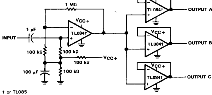
FIGURE 26. AUDIO DISTRIBUTION AMPLIFIER
