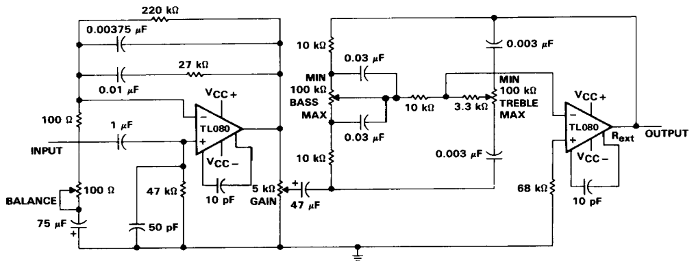
FIGURE 29. IC PREAMPLIFIER
