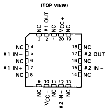
TL082M . . . FK CHIP CARRIER PACKAGE
